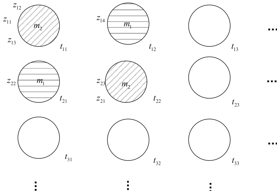
Figure 2 Illustration of the Chinese restaurant metaphor. Tables of the same pattern are grouped into the same cluster.
